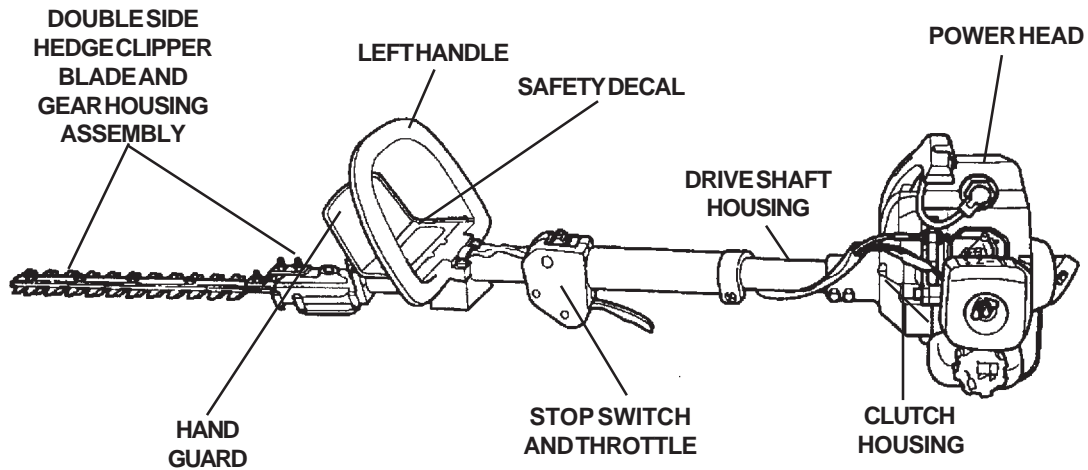
SHC-1700 SHOWN
